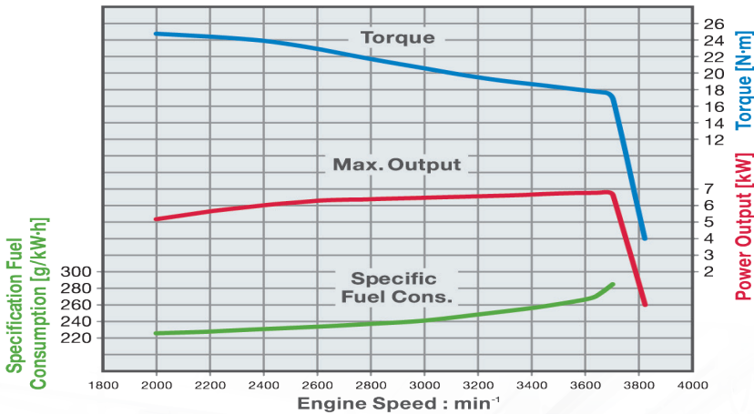
PERFORMANCE CURVES L100W6
